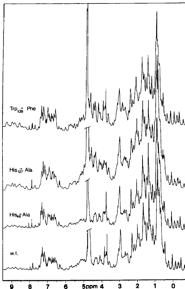
Fig.1. 500 MHz 1 H-NMR spectra of IL-1 \alpha and single amino acid substitution mutants at 25°C.
