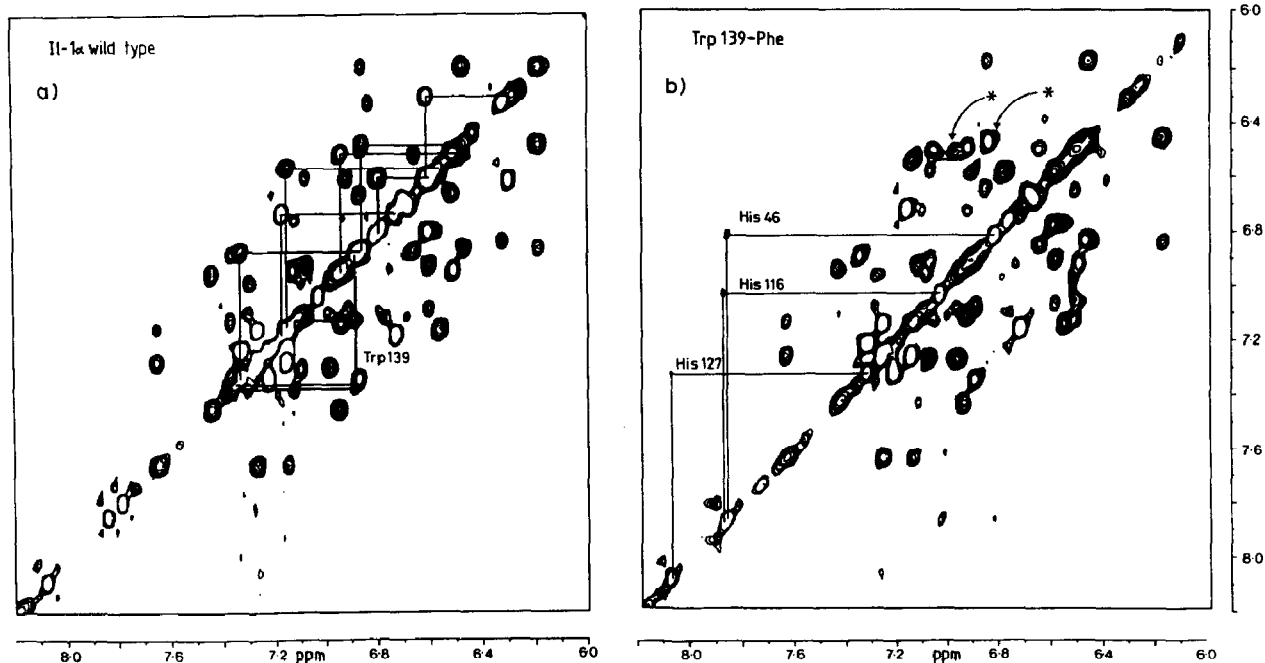
Fig.2. Aromatic region of the pure phase absorption HOHAHA spectra of wild-type IL-1 \alpha (a) and the Trp 139 \rightarrow Phe mutant (b) at 25°C. Some spin system connectivities are indicated by connecting lines. In panel a Tyr spin systems are indicated above the diagonal and the Trp 139 spin system below. The His spin systems are indicated in panel b. The mixing times were 31 ms (a) and 39 ms (b).
